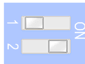
Software C
