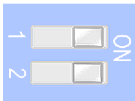
Software A
