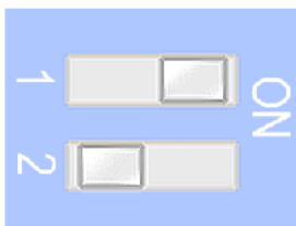
Software B
